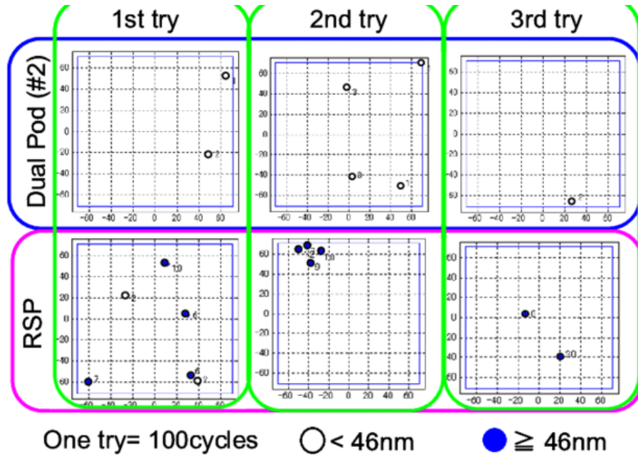
Fig.3 Adder map during transfer experiments using CrN-substrate.
